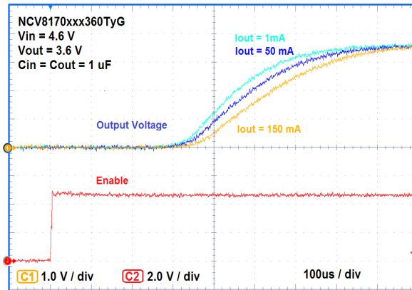
Figure 43. Enable Turn-on Response at V_{out} = 3.6\text{ V}
