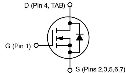
N-CHANNEL MOSFET
