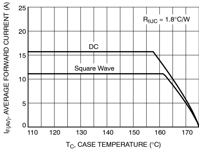
Figure 6. Current Derating
