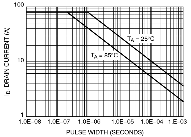
Figure 16. Avalanche Characteristics
