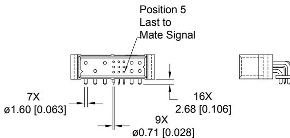
CONNECTOR DIMENSIONS
