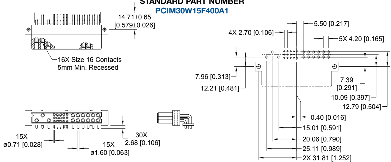
CONNECTOR DIMENSIONS
