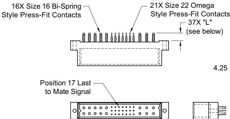
CONNECTOR DIMENSIONS
