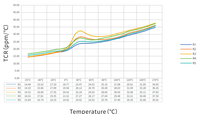
TCR Test Curve - PEWF2512 1.5mΩ
