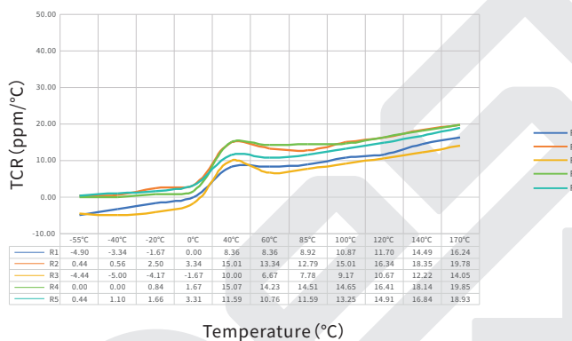
TCR Test Curve - PEWF2512 3mΩ
