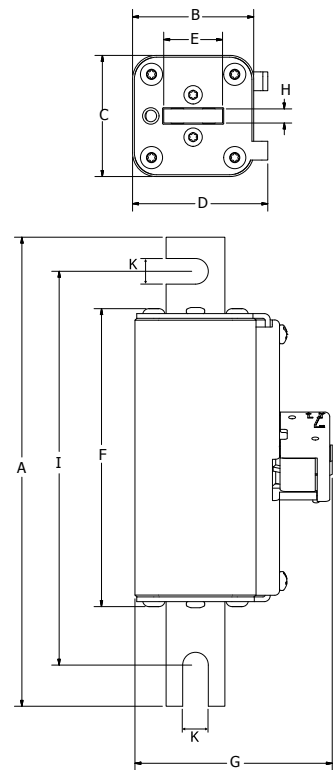
Figure 3. DIN-blade style
