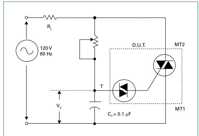
Figure 9: Test Circuit
