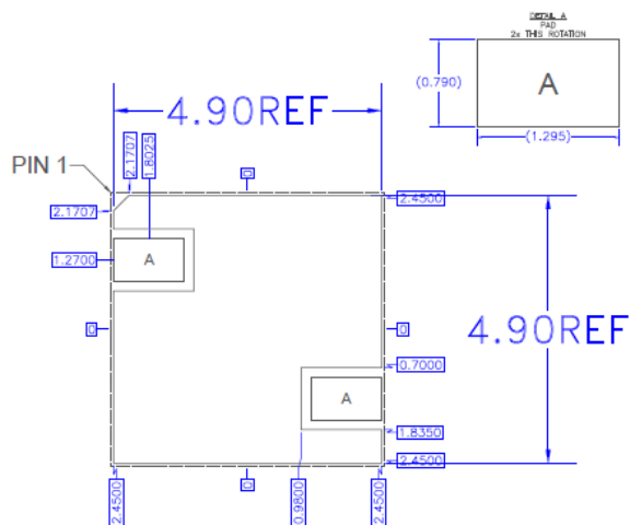
RECOMMENDED LAND PATTERN MASK
