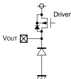
< V_{OUT} Pin>
