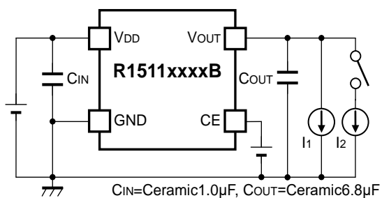
R1511xxxxB Test Circuit for Load Transient Response
