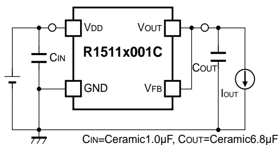
R1511x001C Basic Test Circuit
