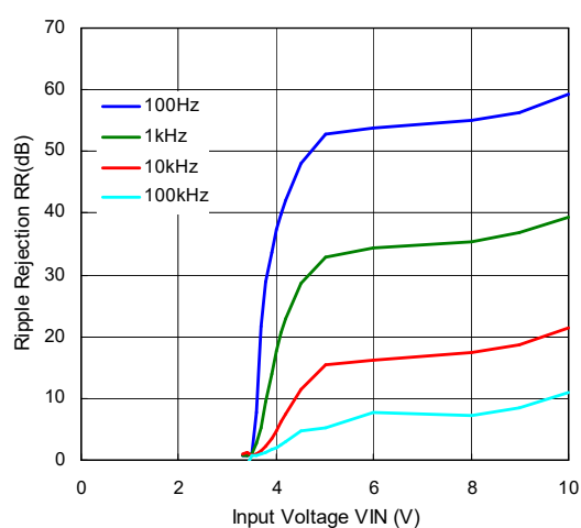
R1518x33xx ( I_{OUT} = 300\text{ mA} )
