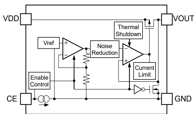
RP123xxxxD Block Diagram
