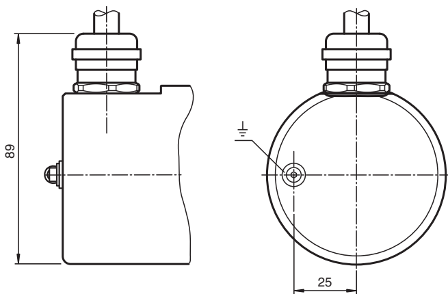
Radial output
