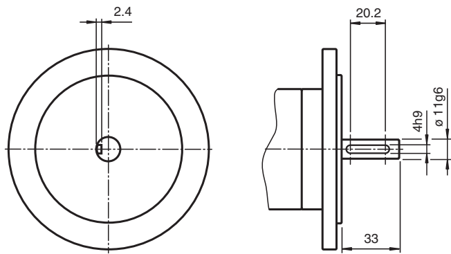
Shaft: 11 mm
