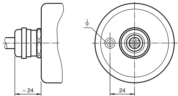
Axial output
