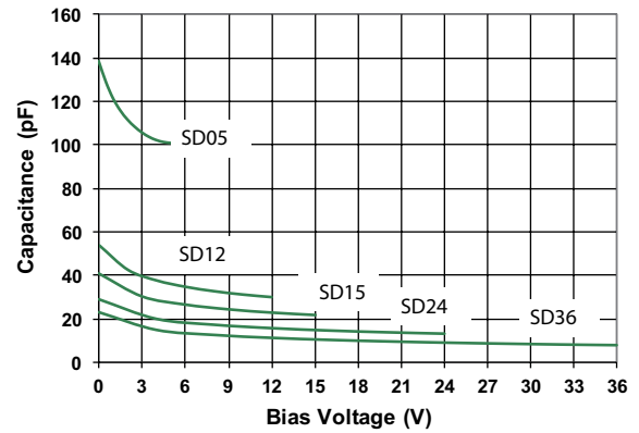
Capacitance vs. Bias
