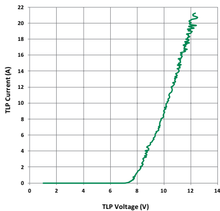
SD05 Transmission Line Pulsing(TLP) Plot
