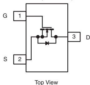
SC-70 (3-LEADS)
