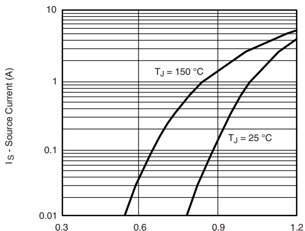
V_{SD} - Source-to-Drain Voltage (V) Forward Diode Voltage vs. Temperature
