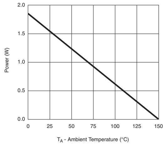
Power, Junction-to-Ambient
