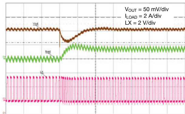
Load Step PWM: 0 A to 1.5 A Load (undershoot)
