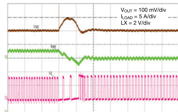
Load Step PWM 0 A to 3 A Load (overshoot)
