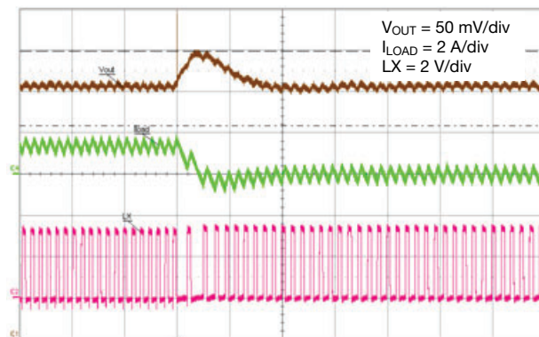
Load Step PWM 0 A to 1.5 A Load (overshoot)
