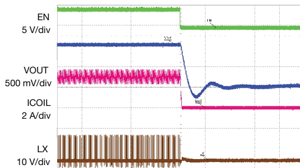
Fig. 17 - Shut-Down, I_{OUT} = 3\text{ A} , Time = 50 μs/div
