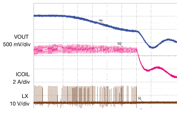
Fig. 18 - Over Current Protection, I_{VALLEY} = 4\text{ A} , Time = 20 μs/div
