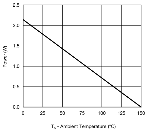
Power, Junction-to-Ambient
