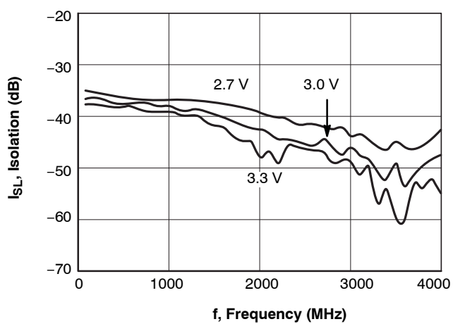
Figure 6. I_{SL} - f
