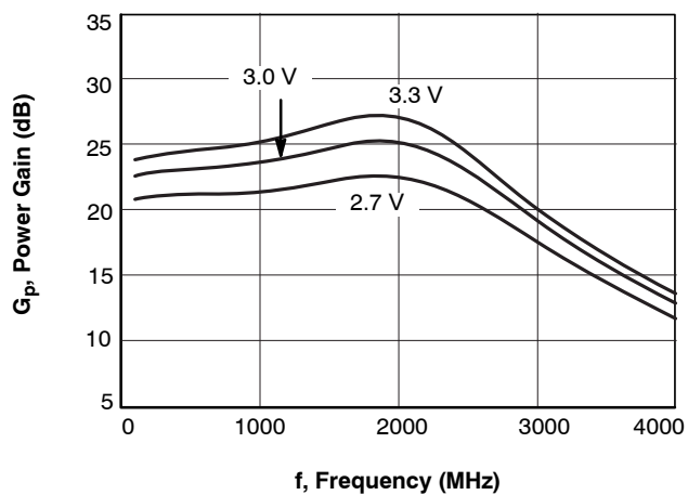
Figure 4. G_p - f
