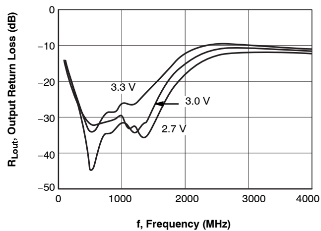
Figure 7. R_{Lout} - f
