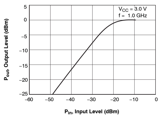
Figure 8. P_{out} - P_{in}
