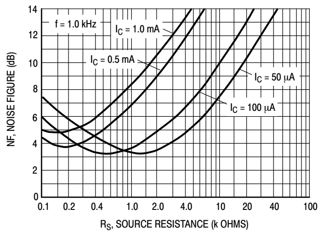
Figure 11. Noise Figure
