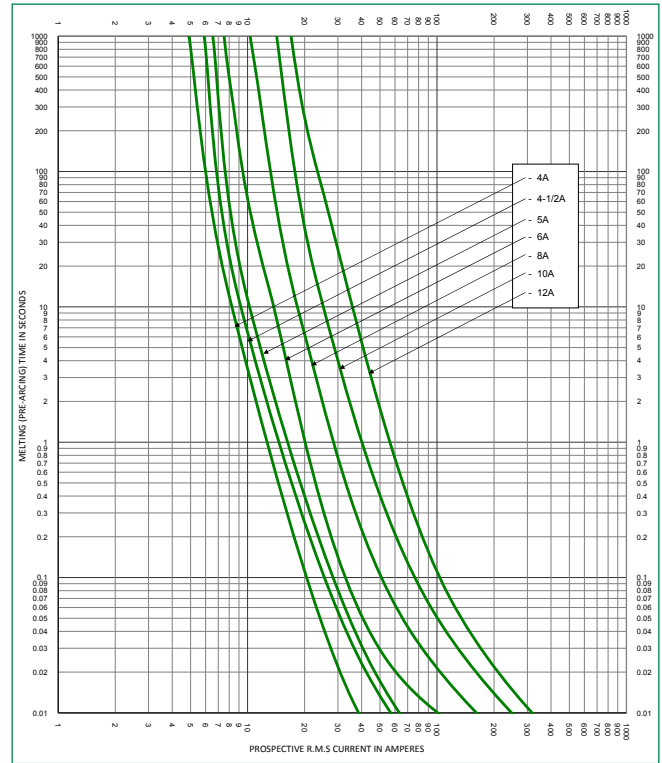
Time Current Curve (4–12 A)
