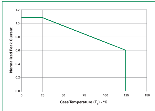
Figure 10: Peak Capacitor Discharge Current Derating
