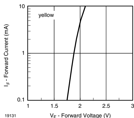
Fig. 20 - Forward Current vs. Forward Voltage
