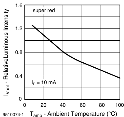
Fig. 7 - Relative Luminous Intensity vs. Ambient Temperature
