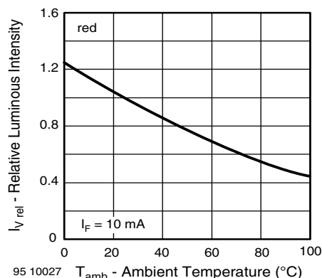
Fig. 12 - Relative Luminous Intensity vs. Ambient Temperature
