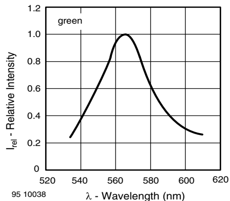
Fig. 18 - Relative Intensity vs. Wavelength
