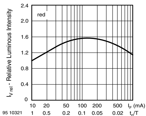
Fig. 11 - Relative Luminous Intensity vs. Forward Current / Duty Cycle
