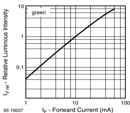
Fig. 20 - Relative Luminous Intensity vs. Forward Current
