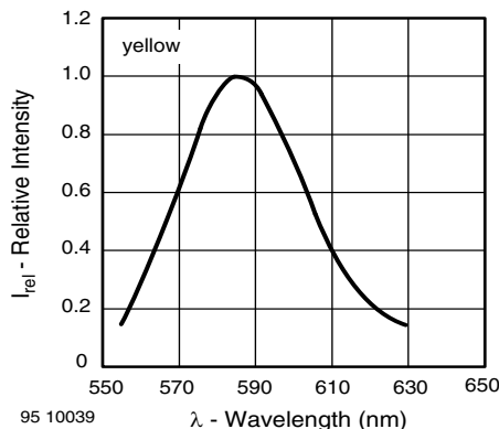
Fig. 13 - Relative Intensity vs. Wavelength
