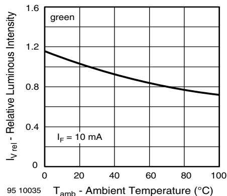
Fig. 22 - Relative Luminous Intensity vs. Ambient Temperature
