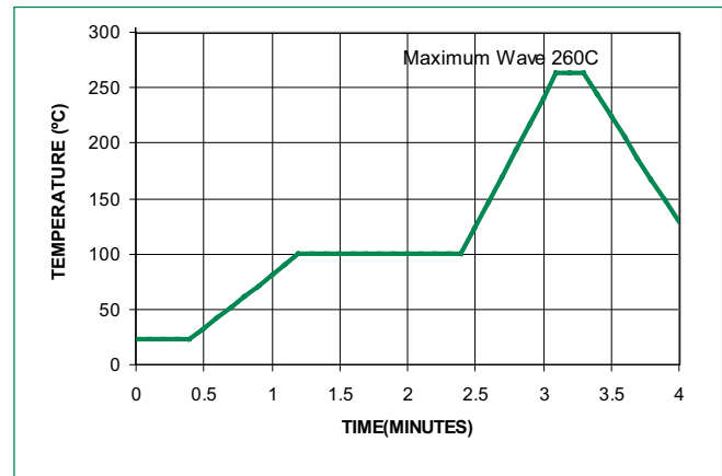
Figure 8. Lead-free Profile
