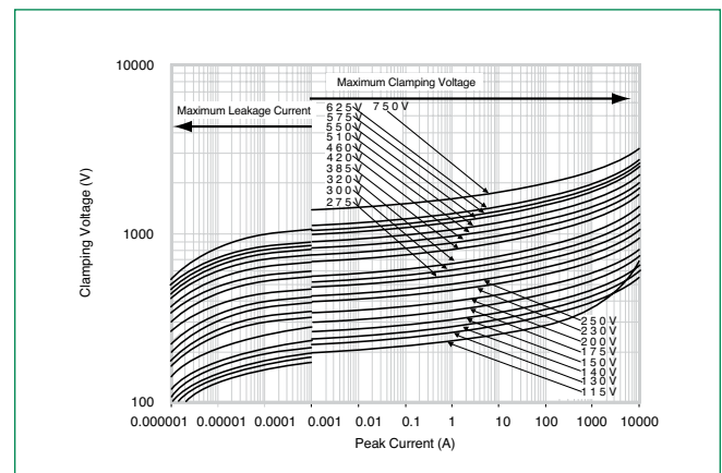
Figure 4. Maximum Clamping Voltage for 20mm Parts
