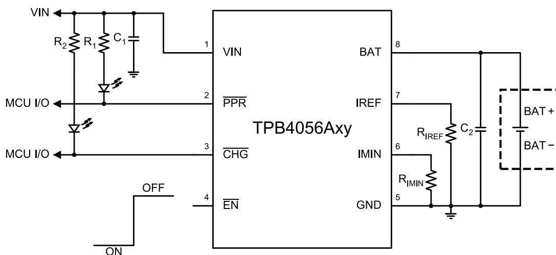
Figure 8 TPB4056A Typical Application Circuit
