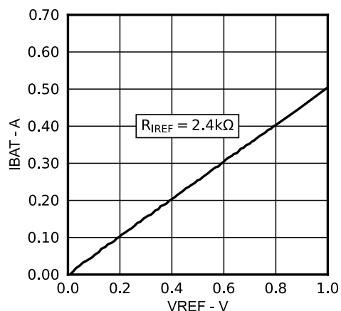
Figure 6 Charging Current IBAT vs IREF Voltage VREF
