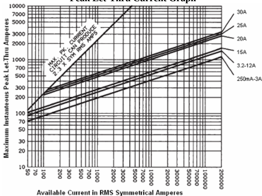
Peak Let-Thru Current Graph
