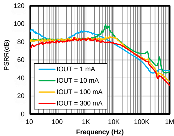
Figure 9 PSRR
