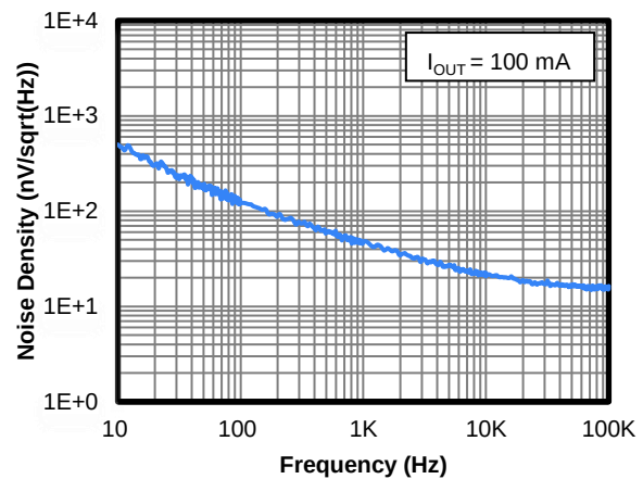
Figure 10 Noise
