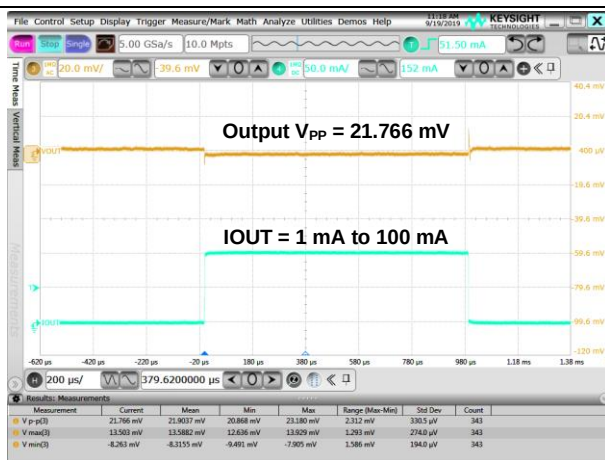
Figure 11 Load Transient
