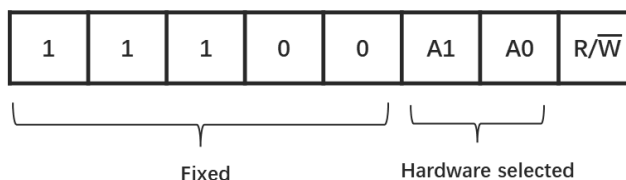
Figure 4. Slave Device Address
