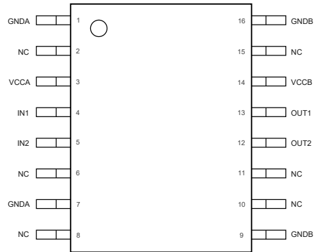
TPT7720 WSOP16 Top View
