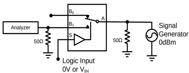
Figure 6 Off Isolation
