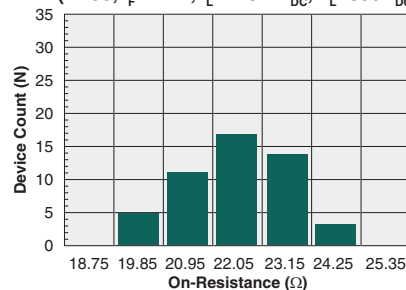
Typical On-Resistance Distribution (N=50, I_F=2\text{mA} , I_L=120\text{mA}_{DC} , V_L=350\text{V}_{DC} )
