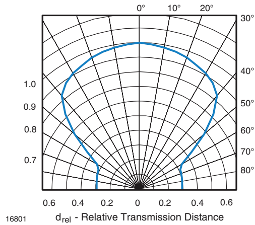
Fig. 11 - Directivity
