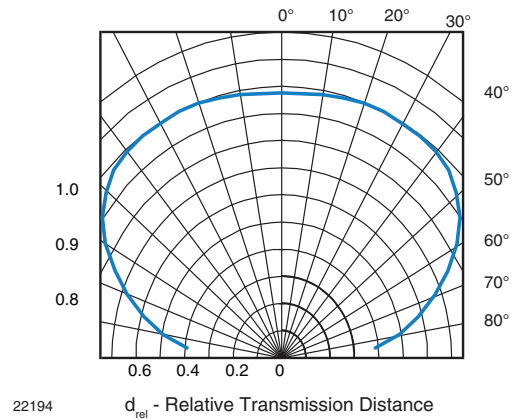
Fig. 12 - Vertical Directivity
