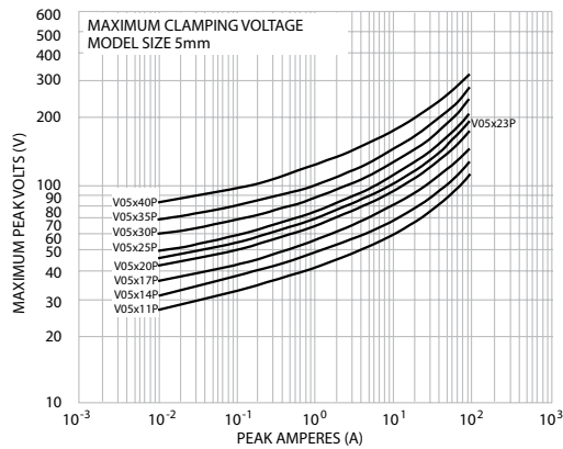
Maximum Clamping Voltage for 5mm Parts V05x11P - V05x40P
