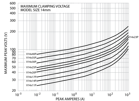
Maximum Clamping Voltage for 14mm Parts V14x11P - V14x40P
