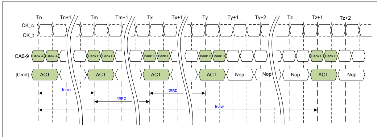
Figure 4 - tFAW Timing
