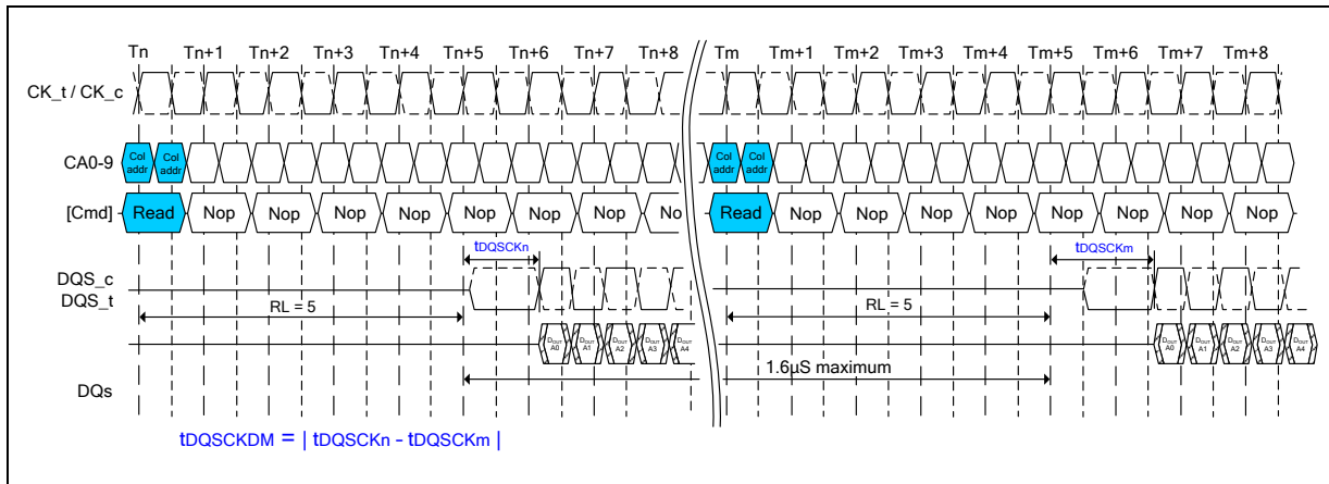
Figure 11 - tDQCKDM timing
