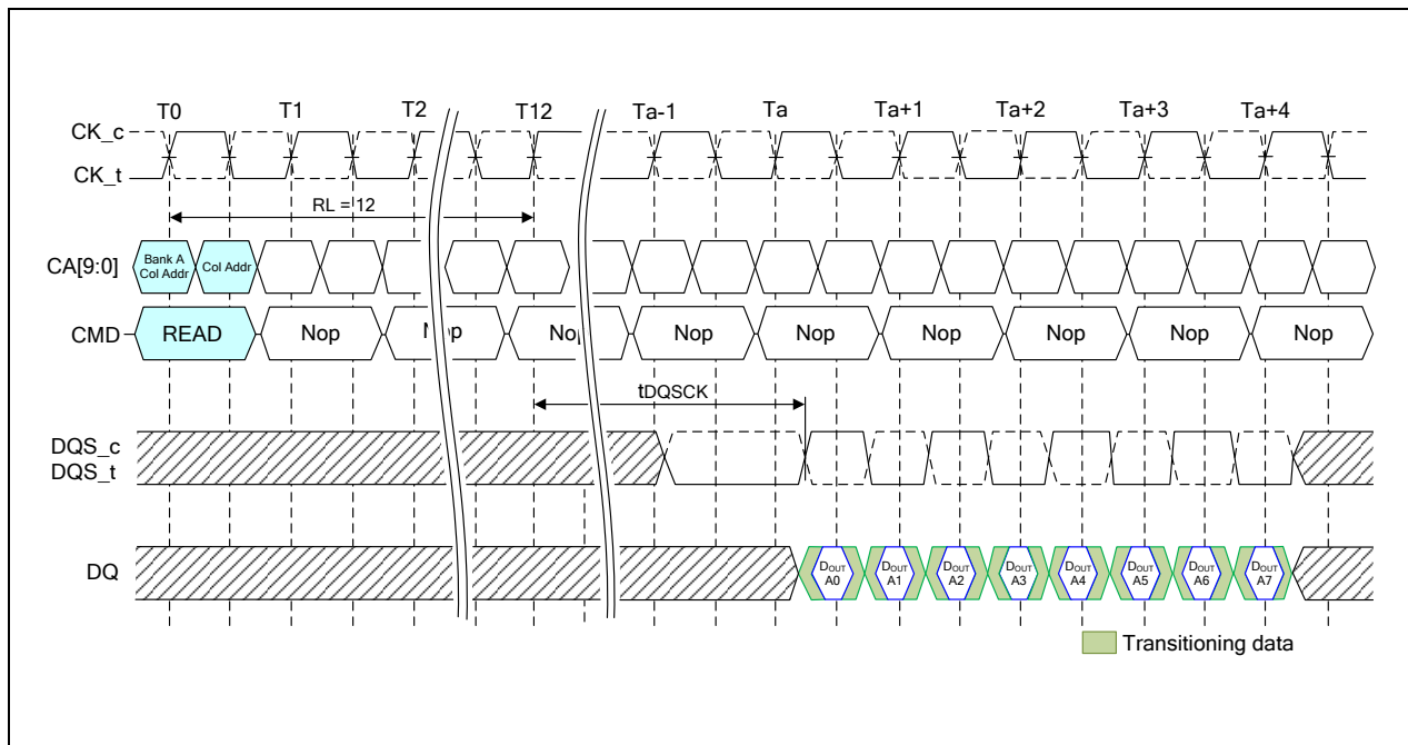
Figure 8 - Burst Read: RL = 12, BL = 8, tDQSCK &gt; tCK
