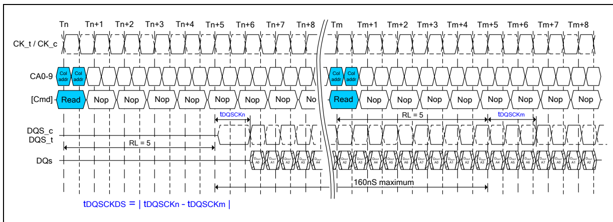
Figure 12 - tDQCKDS timing
