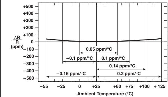
FIGURE 5 - TYPICAL RESISTANCE/TEMPERATURE CURVE (for more details, see table 1)
