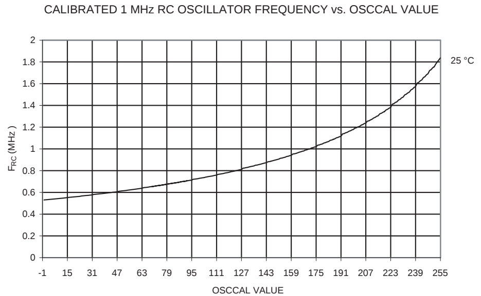
Figure 200. Calibrated 1 MHz RC Oscillator Frequency vs. OSCCAL Value
